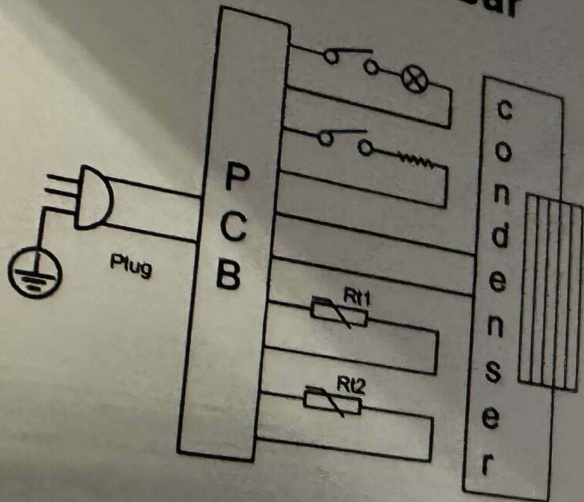
Circuit Diagram
