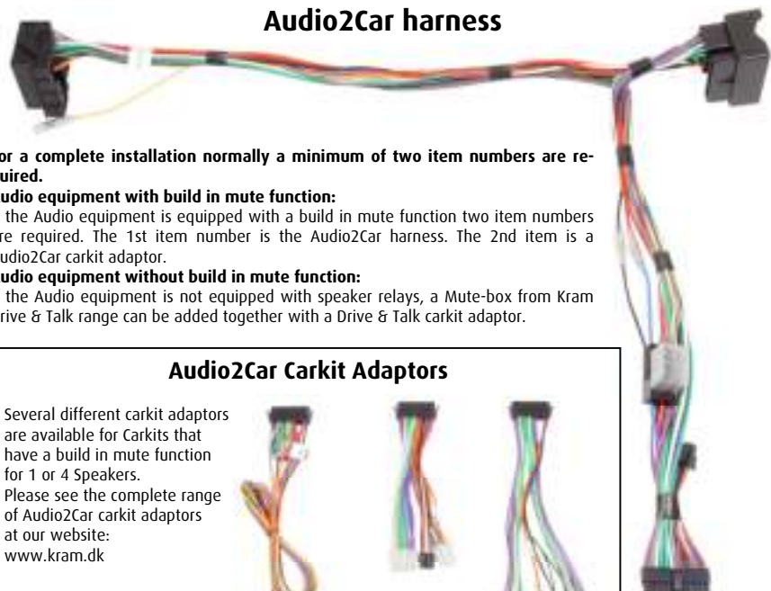
Examples of carkit adaptors
