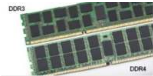
Figure 2. Notch difference
