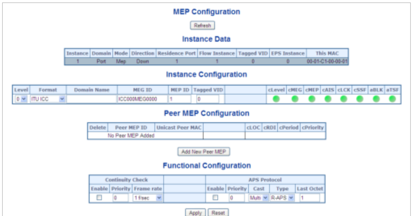
Figure 4-20-2: Detail MEP configuration page screenshot
