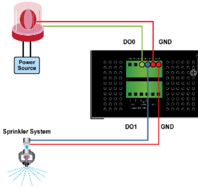
Figure 2-24 Wires DO0 and DO1 to Open Detector
