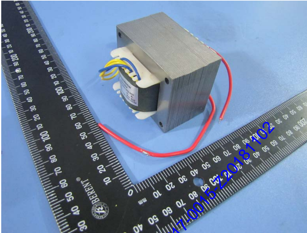
Fig. 11 -- Transformer overview-1
