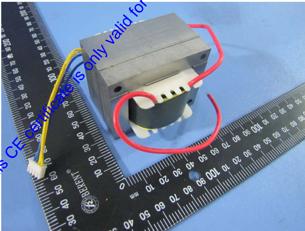
Fig. 12 -- Transformer overview-2
