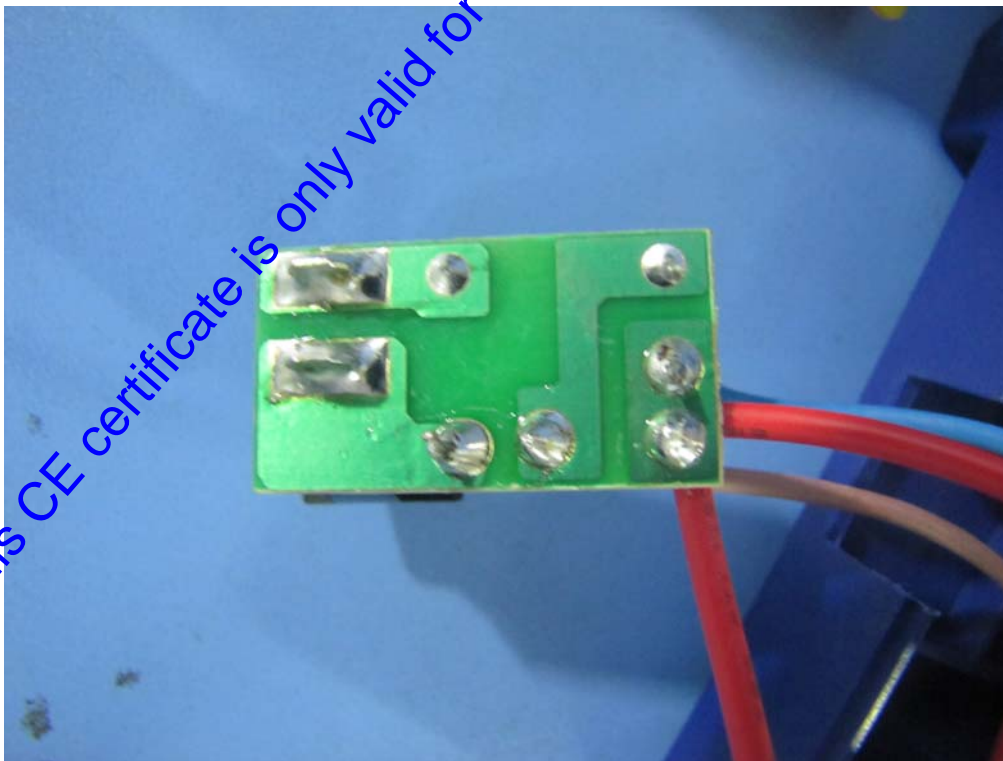
Fig. 16 -- Switch PCB trace side overview
