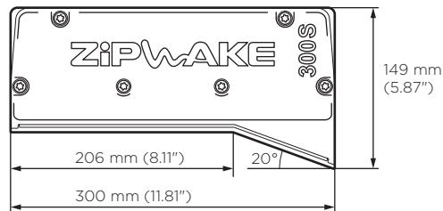
IT300-S CHINE STBD
