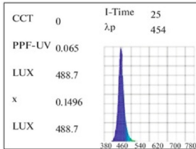
LED (blue)
