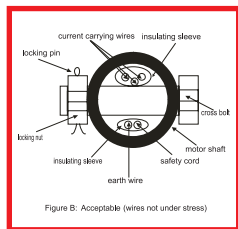
Figure B: Acceptable (wires not under stress)
