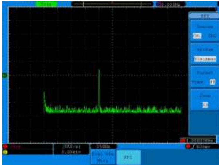
Abb. 24 Blackman-Fenster
