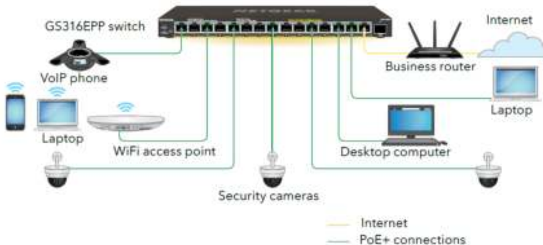
Figure 1. Example connections
