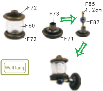
1 Take out F60, F71, F72, F85, and F87 as shown
