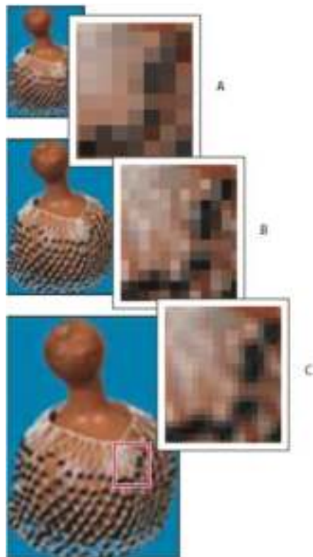
Resampling pixels
