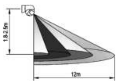
5. Height of installation: 1.8 - 2.5 meters.
