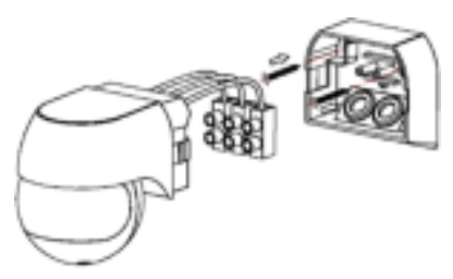
2. Removing the back cover cont.
