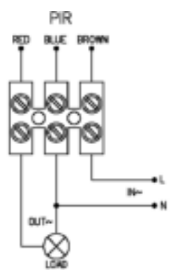
3. Wiring the motion sensor.
