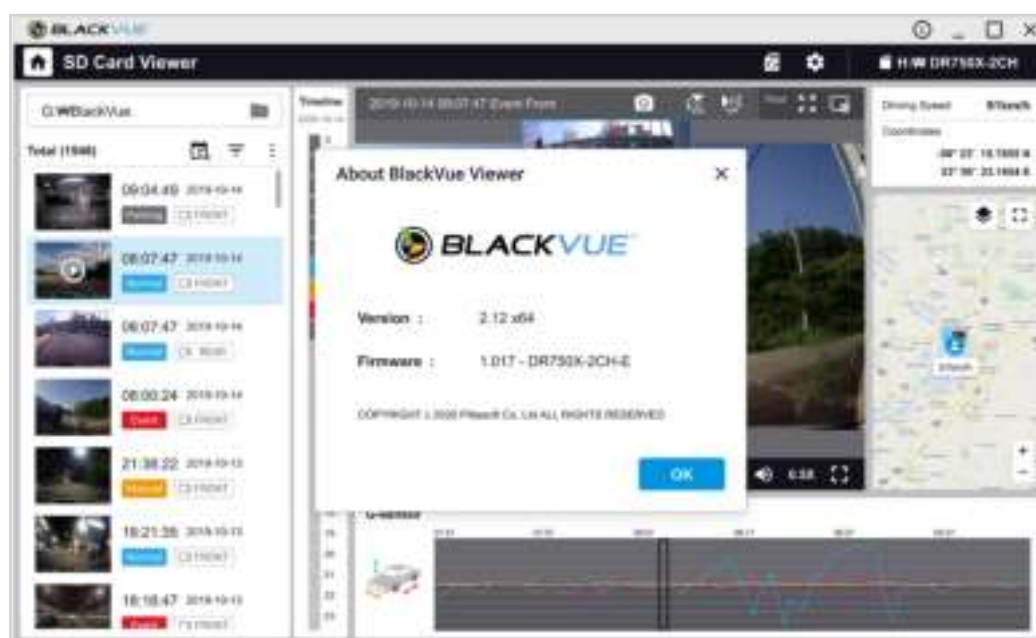
Windows
