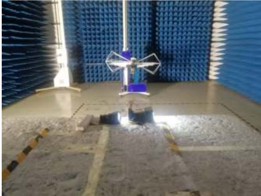
Photo 7 Test scene
