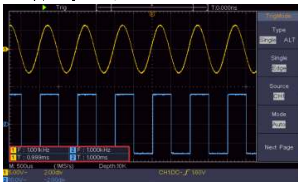
Figure 4-13 Automatic measurement
