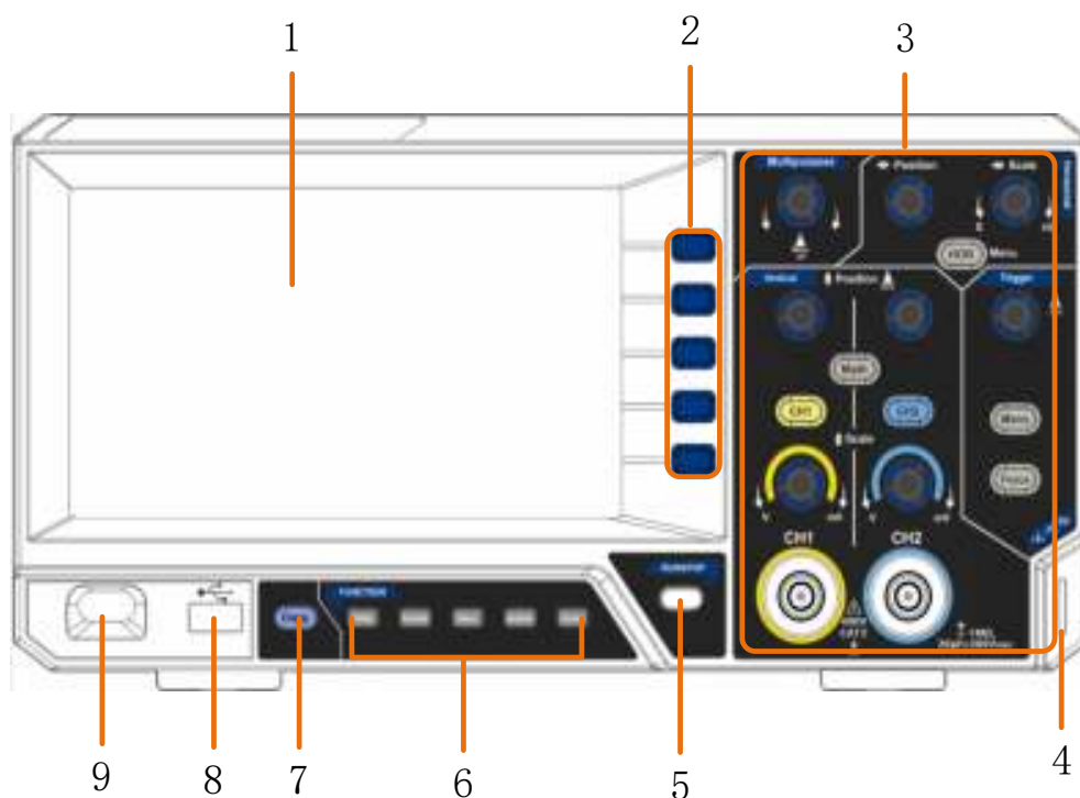
Figure 3-1 Front panel
