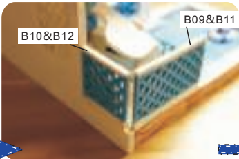
4. glue B10 on B12, glue B09 on B11
