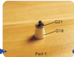
3. glue G18 bottom of G21 to finish part 1
