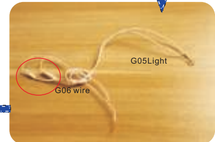
2. connect light G05 and 2pcs 15cm of wire G06
