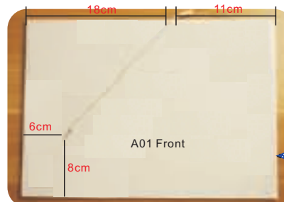
3. glue G01-42, G05 on A01 (refer to the sizes of above picture)
