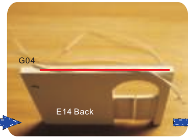
7. along E14 to install wire G04 ( refer to the red line )
