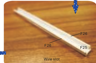
2. glue F26 on both side of F25 to finish the wire slot
