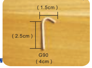
3. refer to above picture to bend G90
