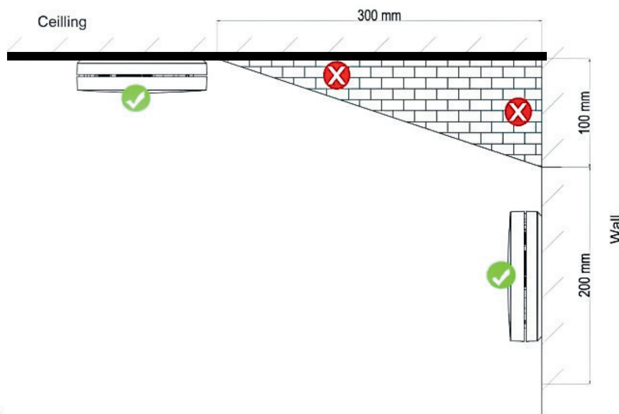
Figure 5: Recommended mounting locations
