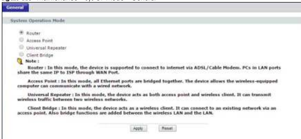
Figure 113 Maintenance > Sys OP Mode > General
