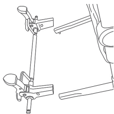
Image 1. Brakes installation
