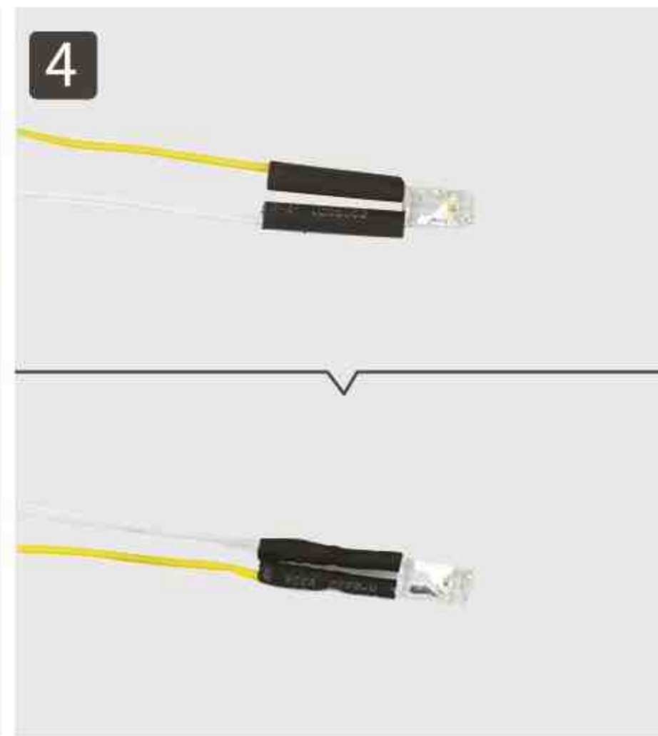
4 Cut the shrinkable tube into 10mm. 2pcs in total. Go through the tube with wires. Heat shrink the tube with flame of lighter.
