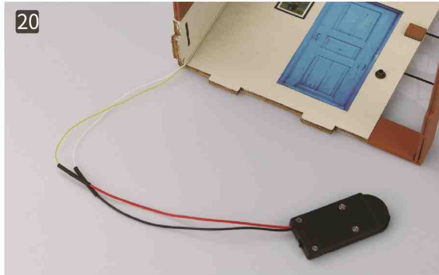
20 Connect the wire of lamp and battery box. Attention: Yellow connect with Red. White connect with black. Test the lamp.
