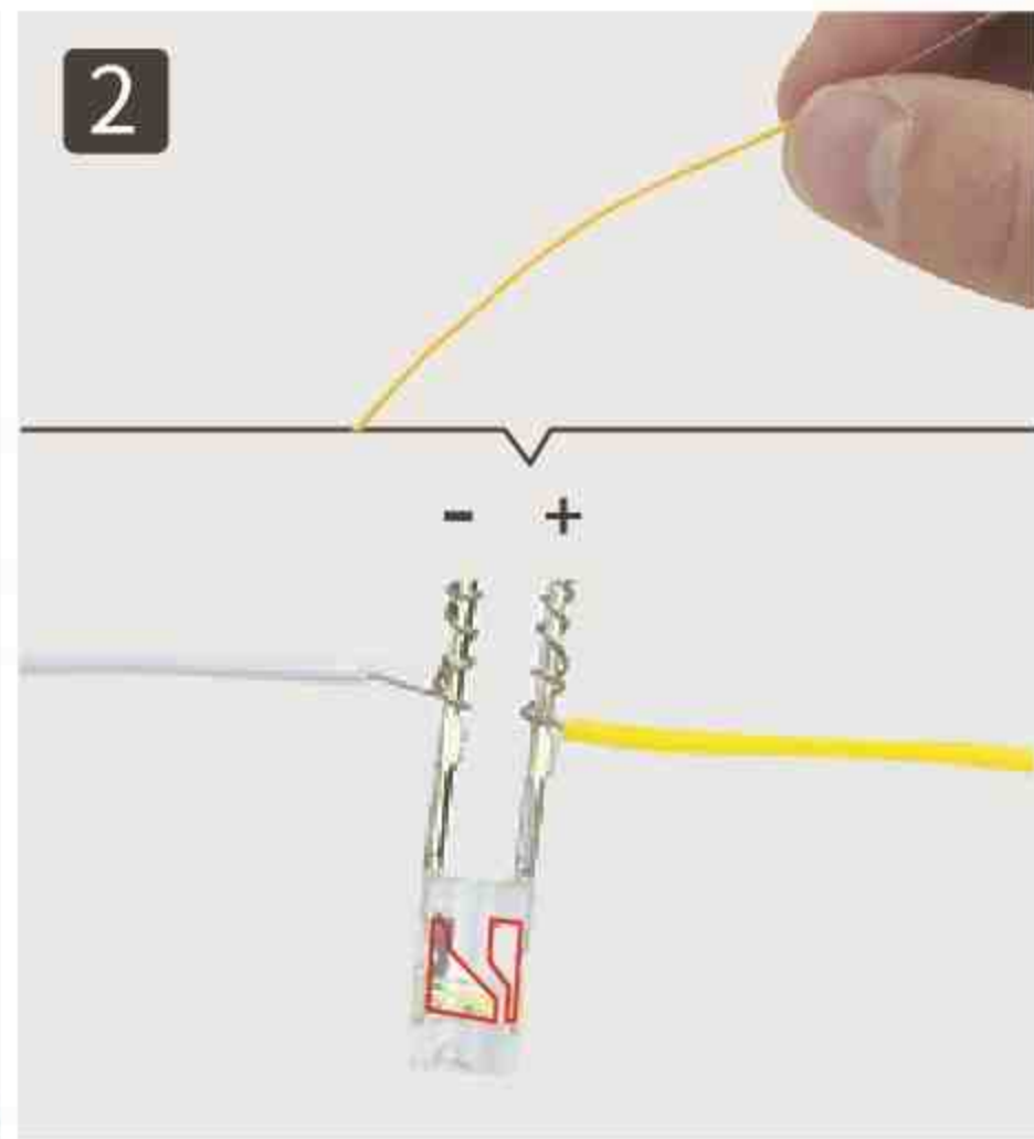
2 Peel off 12mm length rubber from white and yellow wire. Connect to the lamp as shown.
