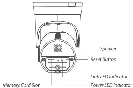
UNDERSIDE VIEW
