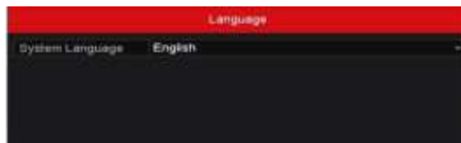
Figure 2-15 Language Configuration
