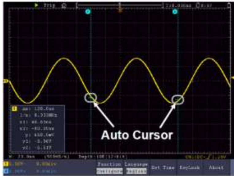
Figure 4-21 Auto Cursor
