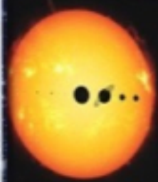
OUR SOLAR SYSTEM
