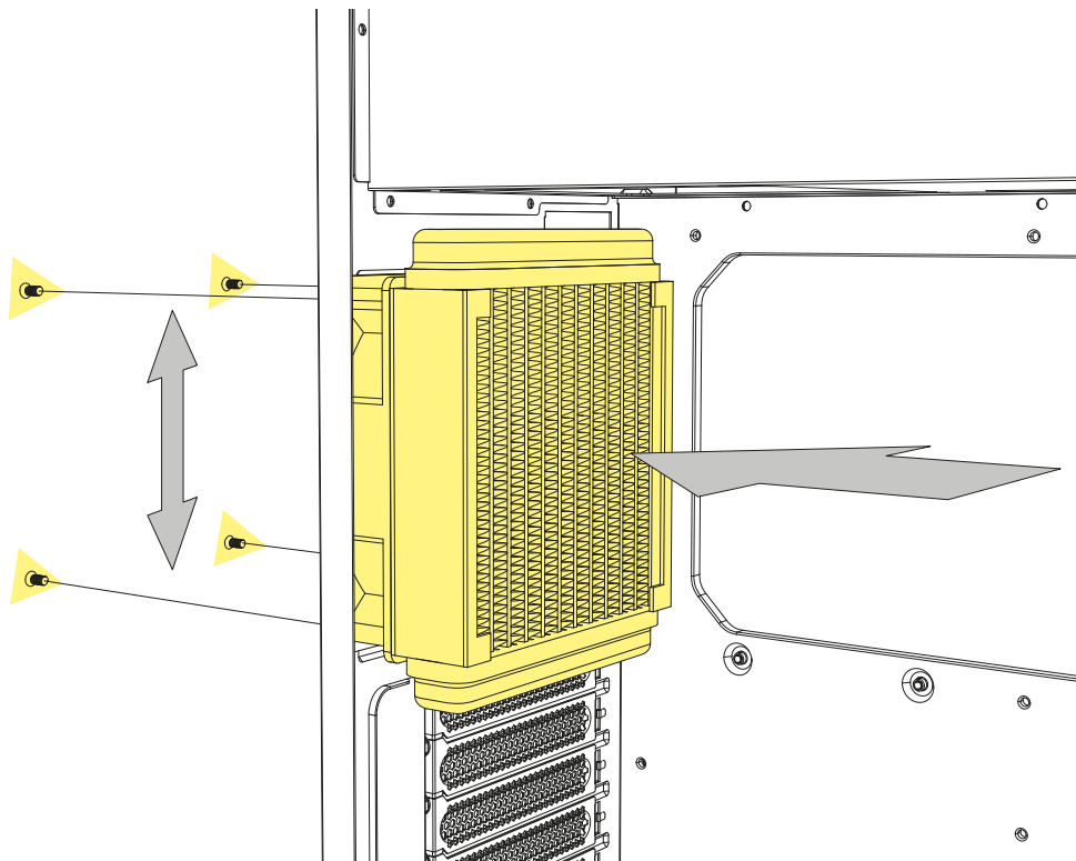
120 mm Radiator
