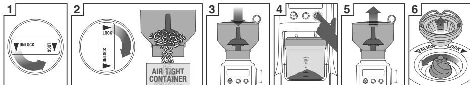
Unlock hopper
