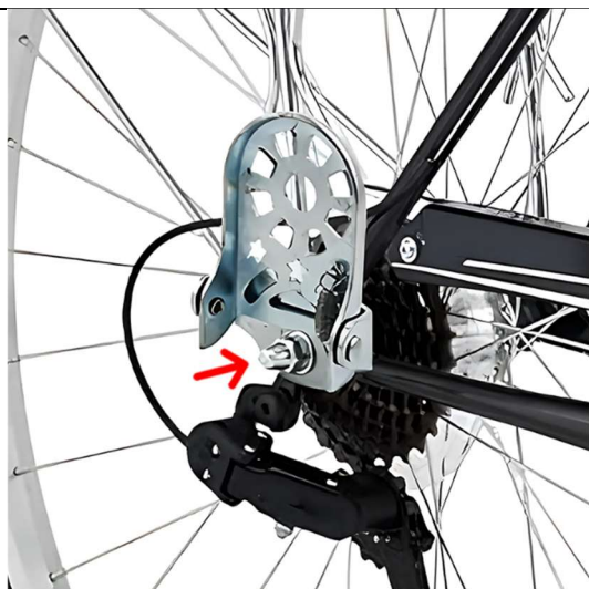
Step 5: Loosen the nut on your rear wheel. Place the footpegs around the bolt and tighten the nut firmly again.
