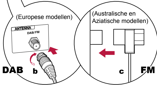
a AM-loop-antenne, b DAB/FM-antenne, c FM-binnenantenne
