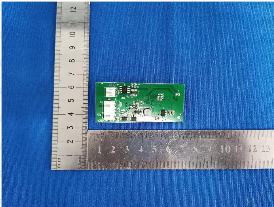
Photo 10: PCB view
