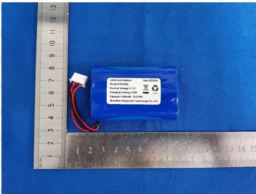
Photo 8: Battery view
