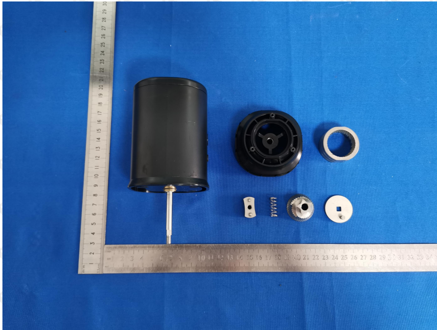
Photo 5: Internal view
