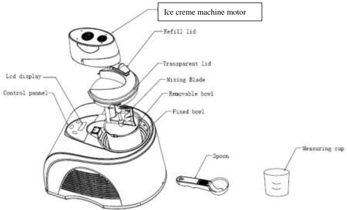
Illustration 1-Exploded View
