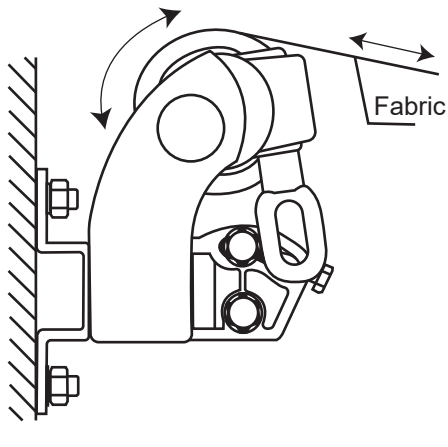
Correct operation
