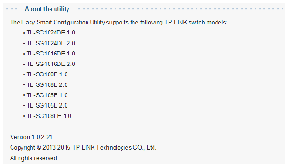
Figure 8-2 Software Version
