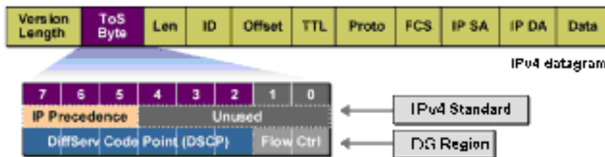
Figure 7-3 IP datagram
