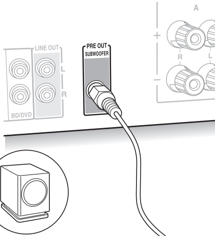
Subwoofer with a built in amplifier
