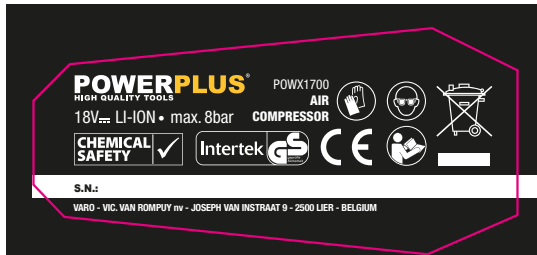
Data Label
