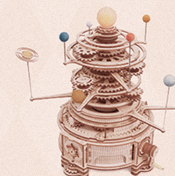
Solar system
