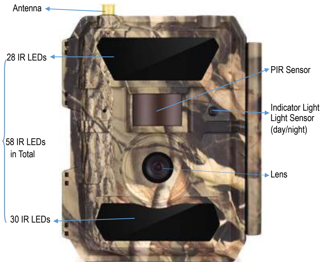
2.1 Figure 1: Front View of Camera;
