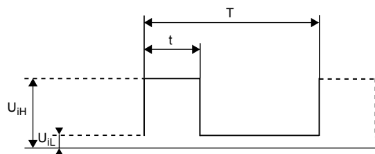
Fig. 15 PWM signal
