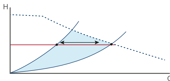
Fig. 13 Constant-pressure curve
