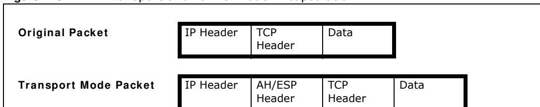
Figure 273 VPN: Transport and Tunnel Mode Encapsulation
