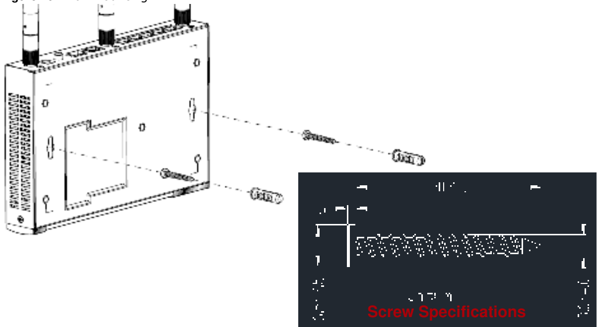
Figure 40 Wall Mounting
