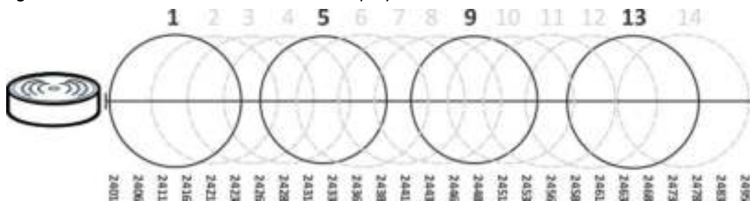
Figure 147 An Alternative Four-Channel Deployment
