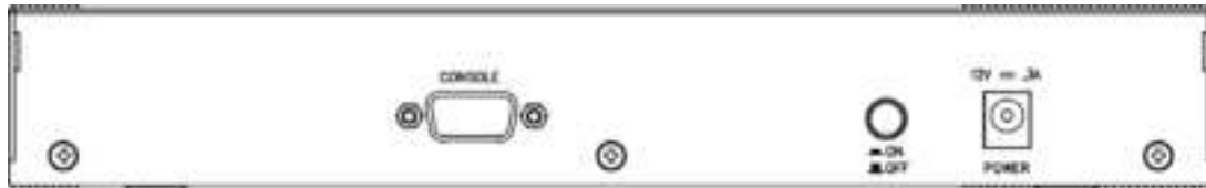
Figure 39 USG60 / USG60W Rear Panel
