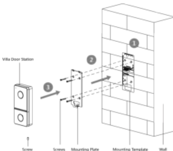
Figure 3-3 Surface Mounting without Protective Shield
