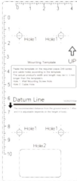
Figure 3-4 Mounting Template
