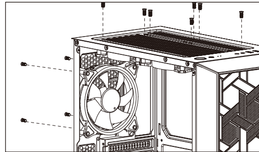
(7b) Install Rear and Top Fan
