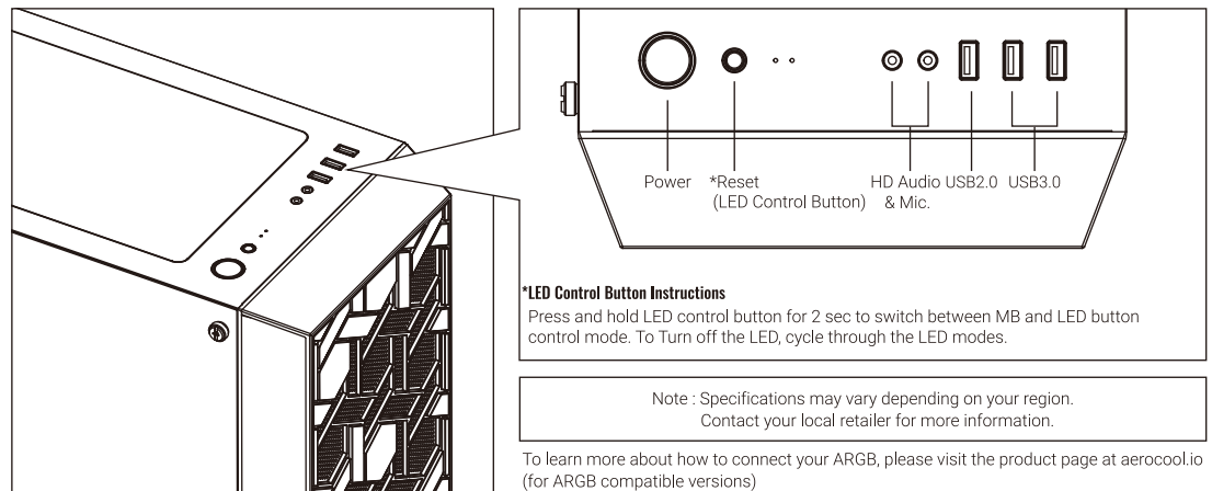
I/O Panel
