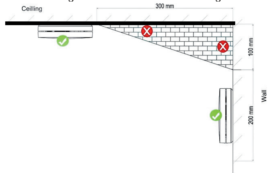
Figure 3: Recommended mounting locations
