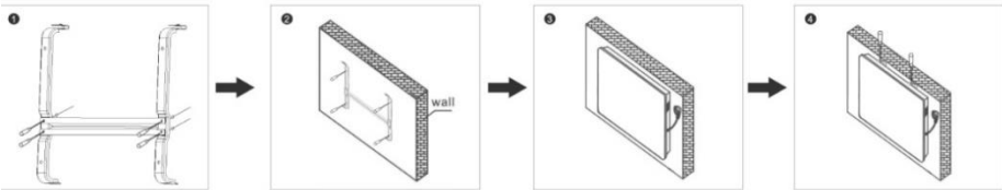
Fig. 2 Wandmontage
