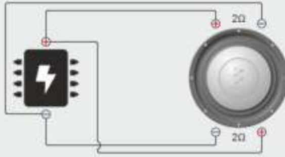
Serial wiring → 4 Ohms
