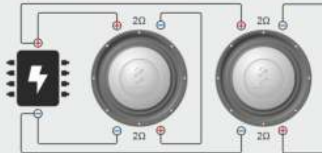
Parallel / serial mixed wiring → 2 Ohms
