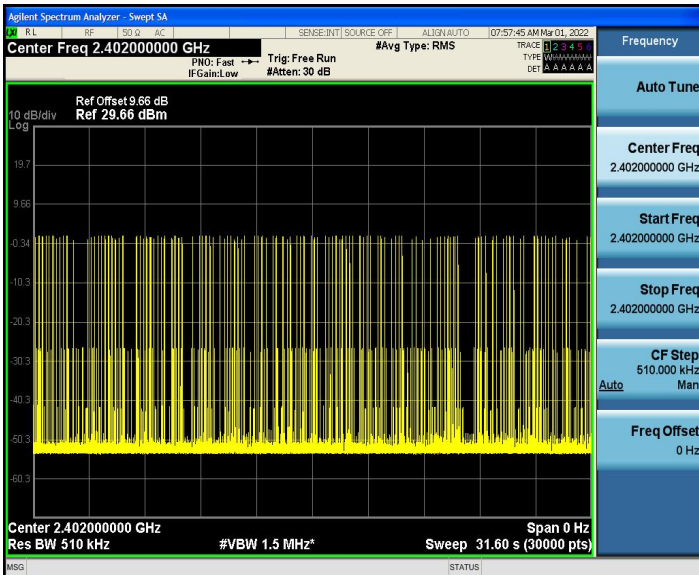
GFSK-DH5: 2402 MHz
