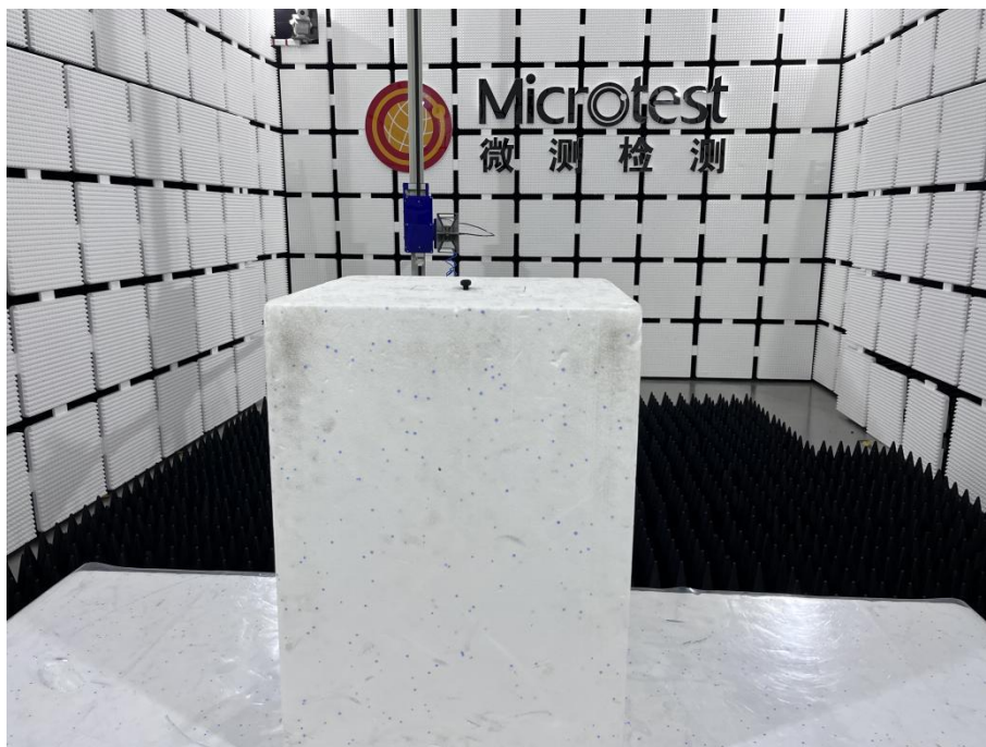
Radiated emissions above 1 GHz-TX
