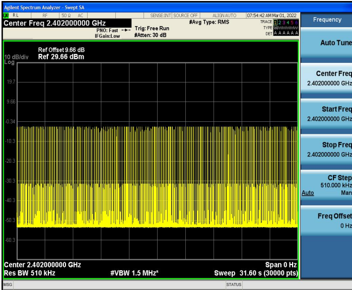
GFSK-DH3: 2402 MHz
