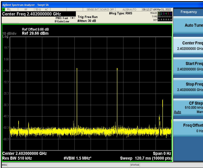
GFSK-DH3: 2402 MHz
