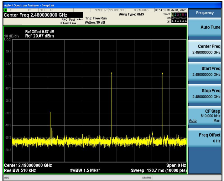
GFSK-DH3: 2480 MHz
