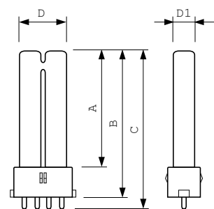
PL-S 5W/827/4P LM
