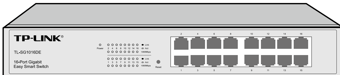
Figure 2-4 Front Panel of TL-SG1016DE
