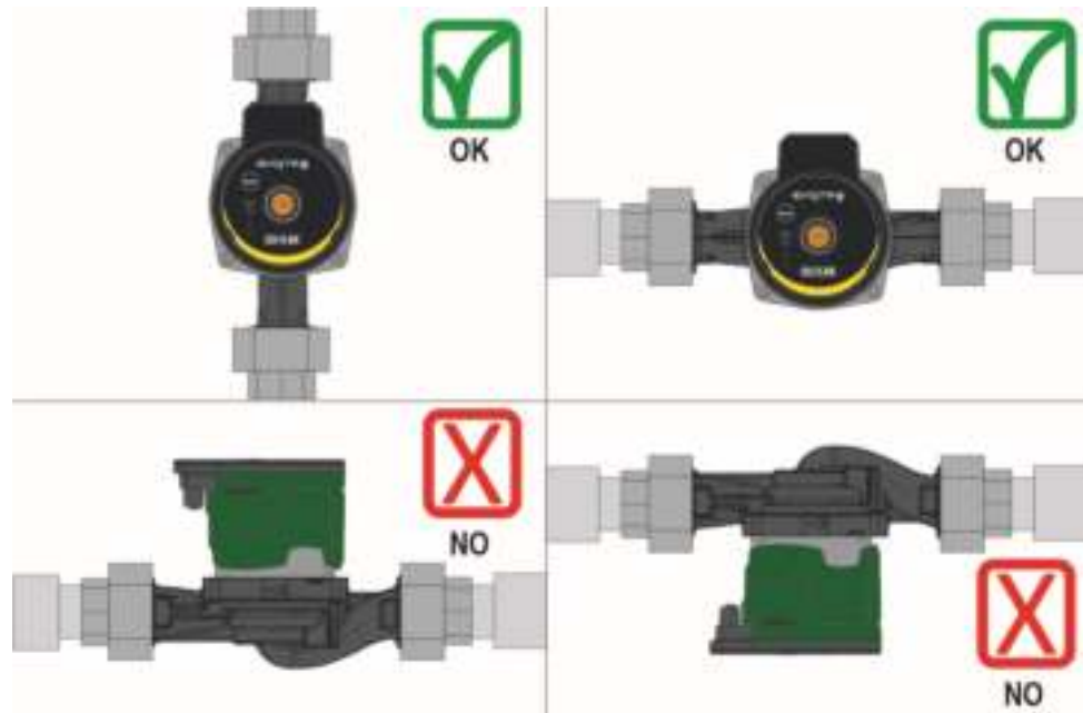
Abb. 13: Montageposition
