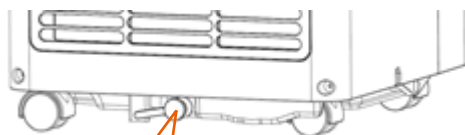
Continuous drain hose (Inner diameter = 16 mm)
