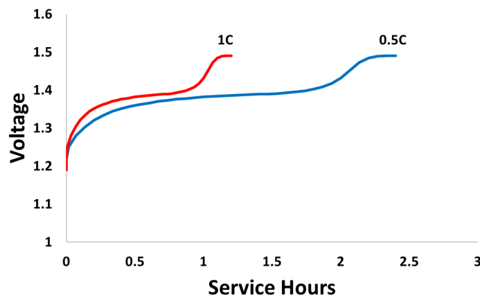
Fast Charge- AAA Value
