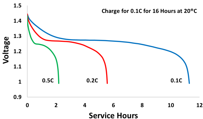
Low Rate Discharge- AAA Value
