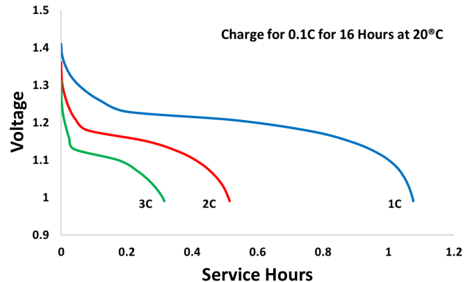
High Rate Discharge- AAA Value
